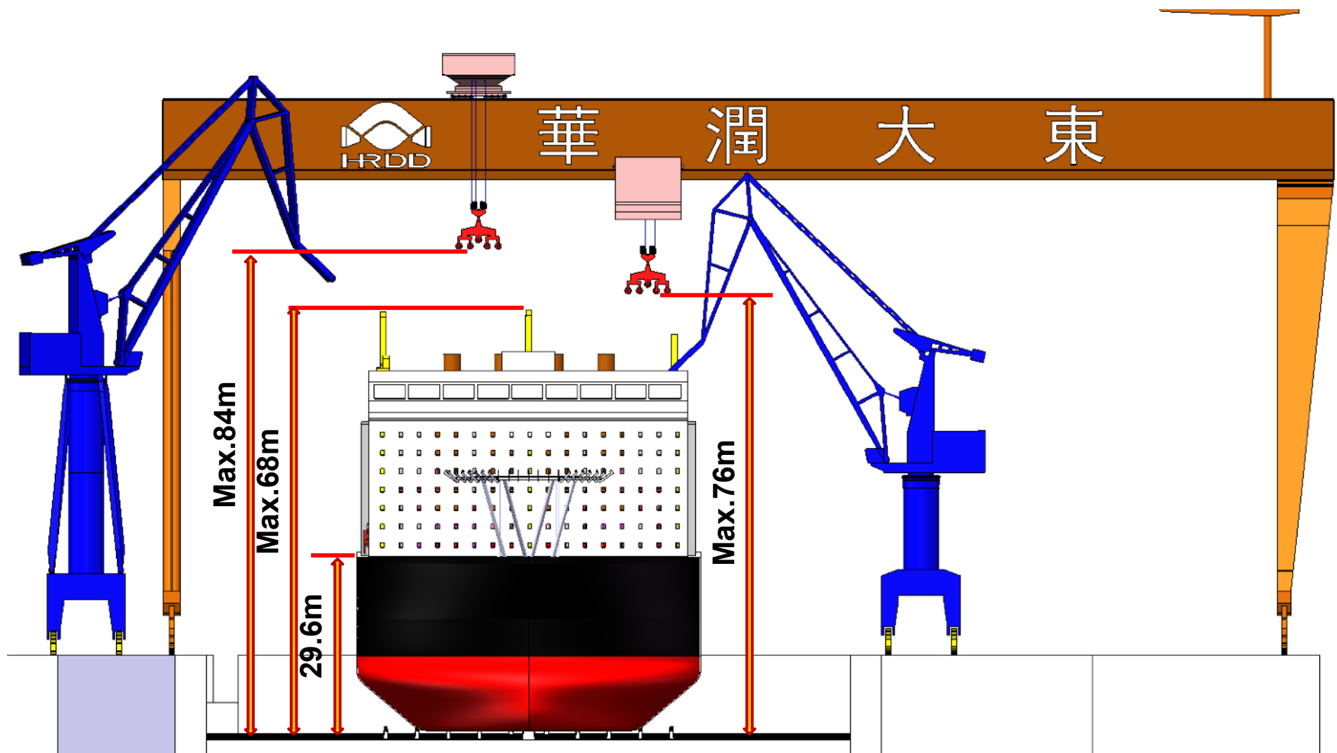
FRONT VIEW
