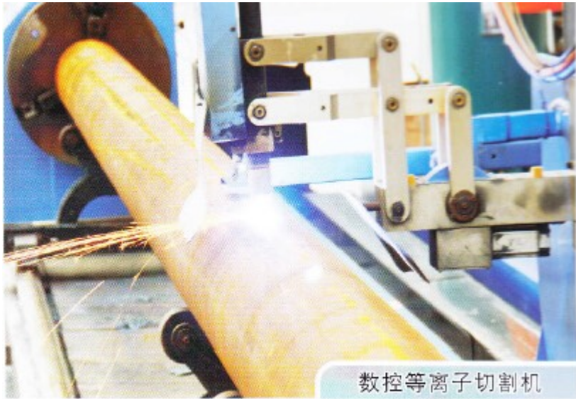
CNC plasma cutter
